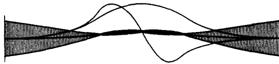
Fig. 11. The optimal design (form and cross-sectional area) of a clamped arch with c = 2 (and p = 3 ) for 0 \leq \bar{\alpha} \leq 0.07 (inactive constraint). The optimal frequency \omega = 77.6 is bimodal, and \omega/\omega_{cu} = 2.24 .
